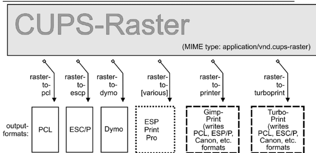
Figure 21.9. Raster to Printer-Specific Formats.
