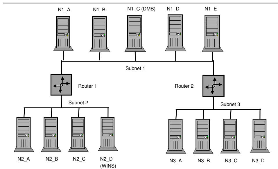
Figure 9.1. Cross-Subnet Browsing Example.
