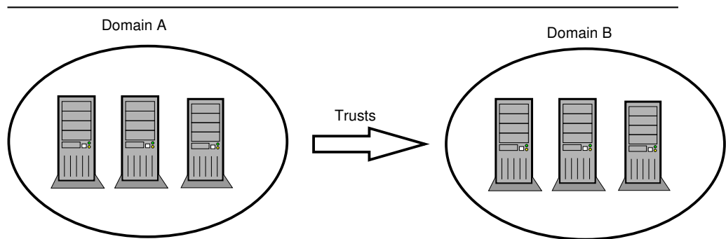
Figure 18.1. Trusts overview.
