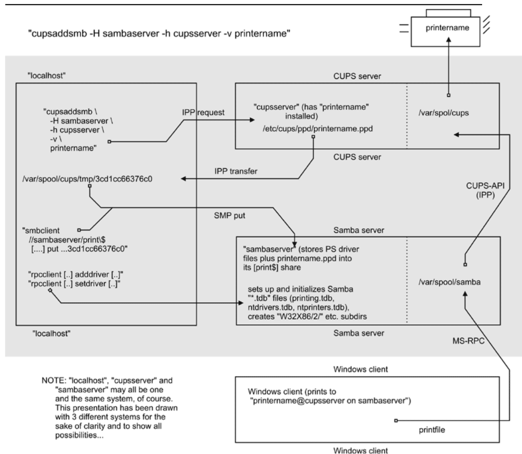
Figure 21.16. cupsaddsmb Flowchart.
