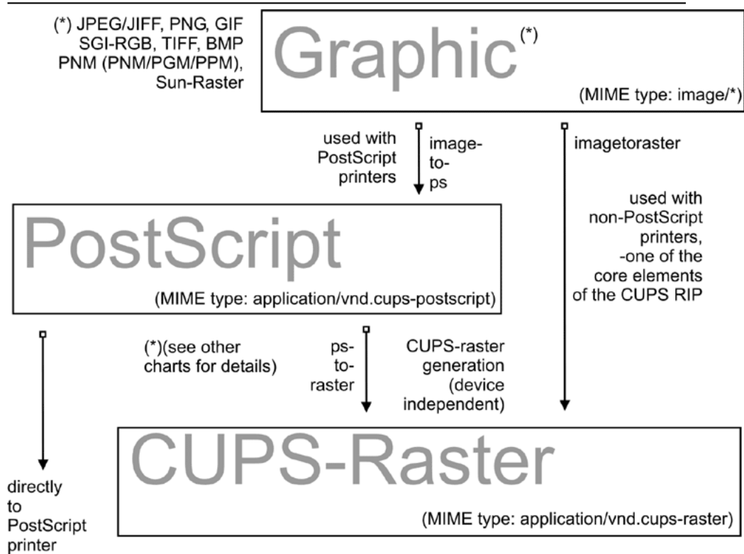
Figure 21.8. Image Format to CUPS-Raster Format Conversion.
