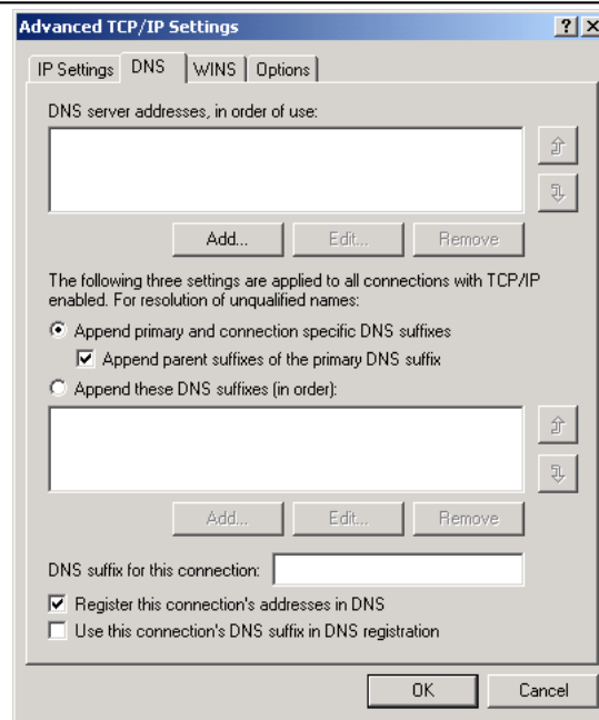
Figure 8.9. DNS Configuration.
