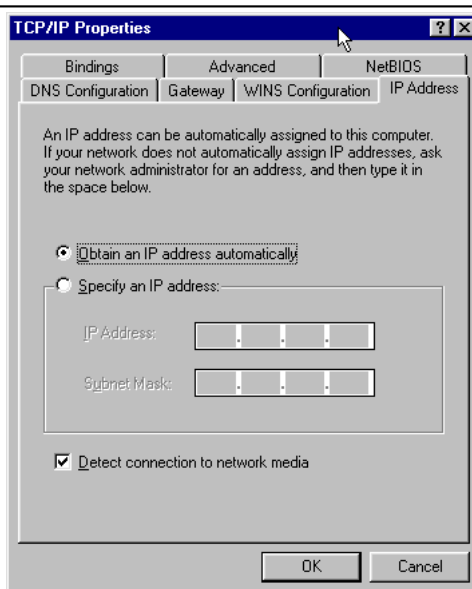
Figure 8.12. IP Address.
