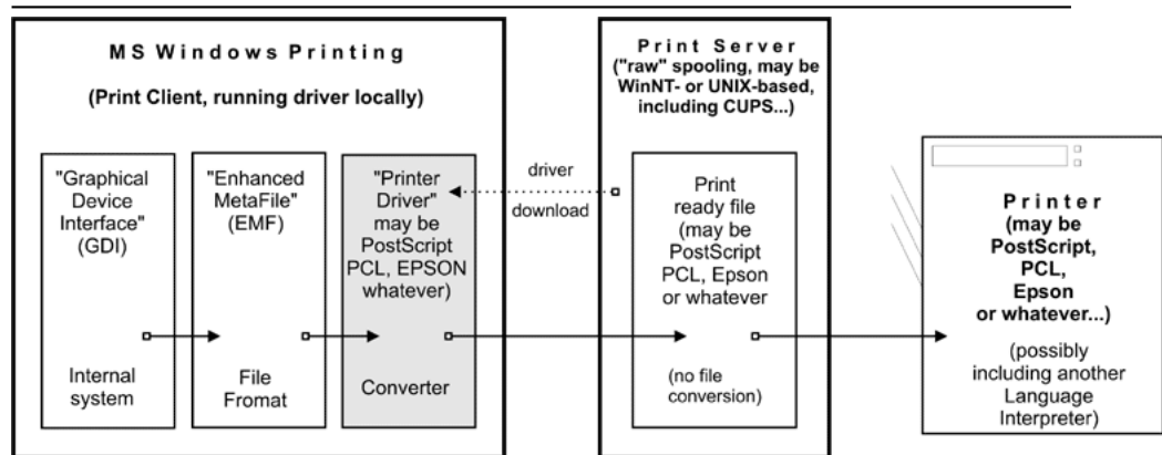
Figure 21.13. Print Driver Execution on the Client.
