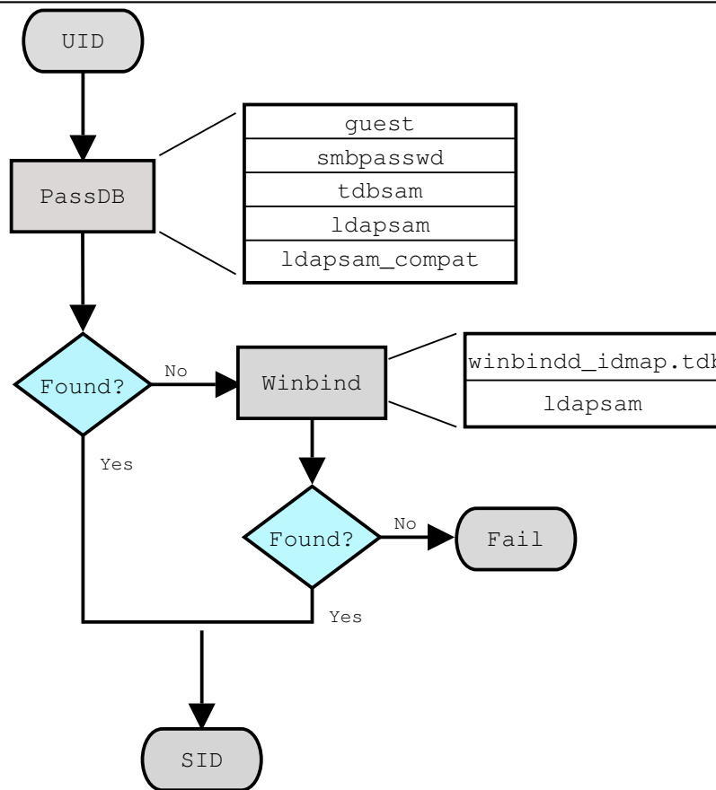
Figure 10.2. IDMAP: Resolution of UIDs to SIDs.
