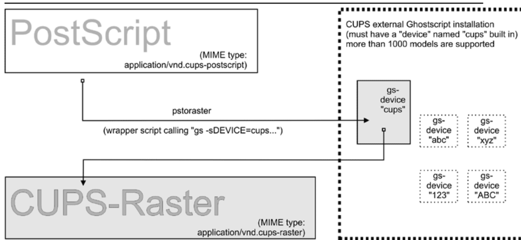
Figure 21.7. CUPS-Raster Production Using Ghostscript.
