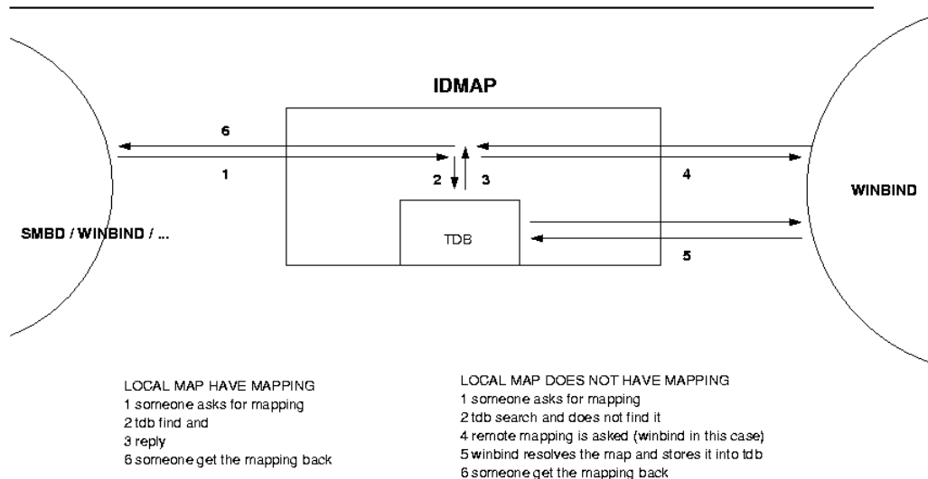
Figure 23.1. Winbind Idmap
